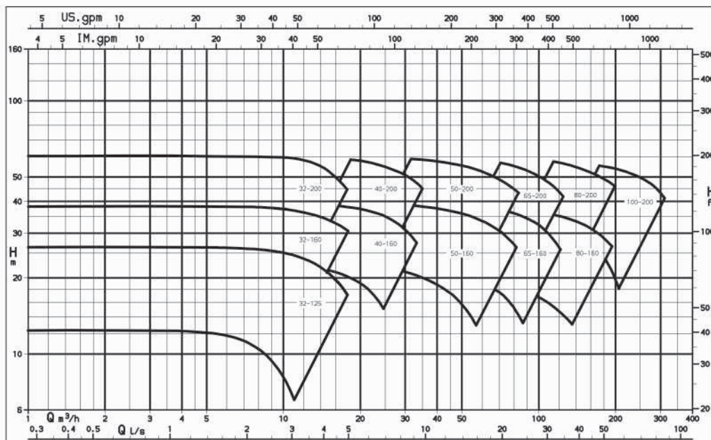
Selection Chart 2900 RPM
